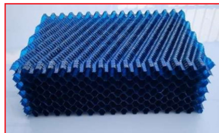
COOLING TOWER PVC FILLS
